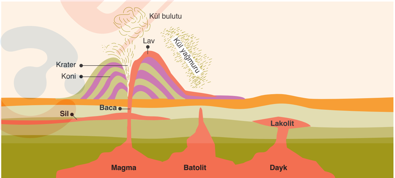
Volkanik arazi
